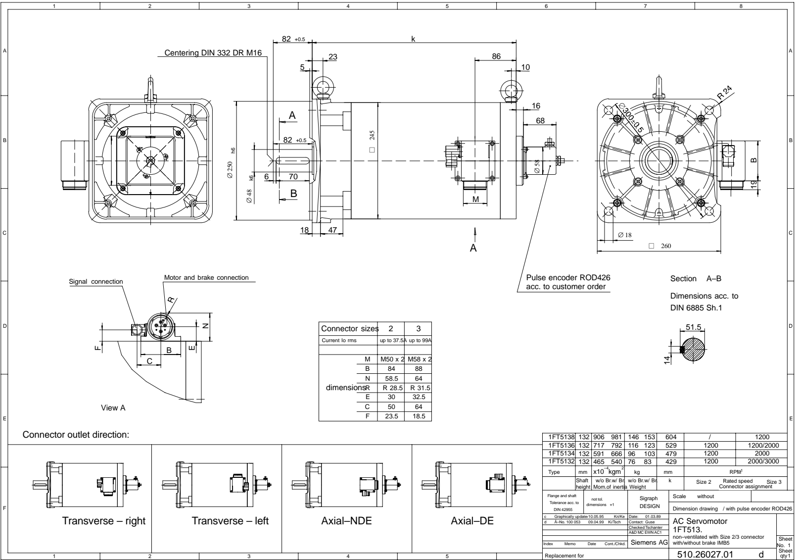
Fig. 4-17 1FT5133 non-ventilated with Size 2/3 connector
